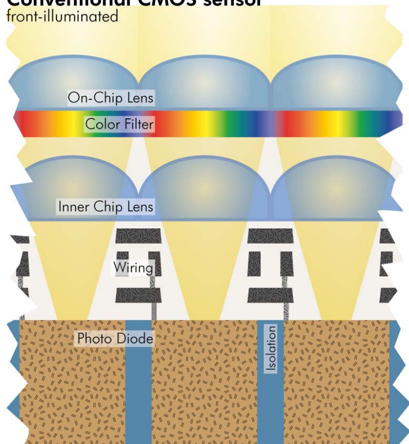
Figure 14: Illustration of conventional CMOS sensor technique
