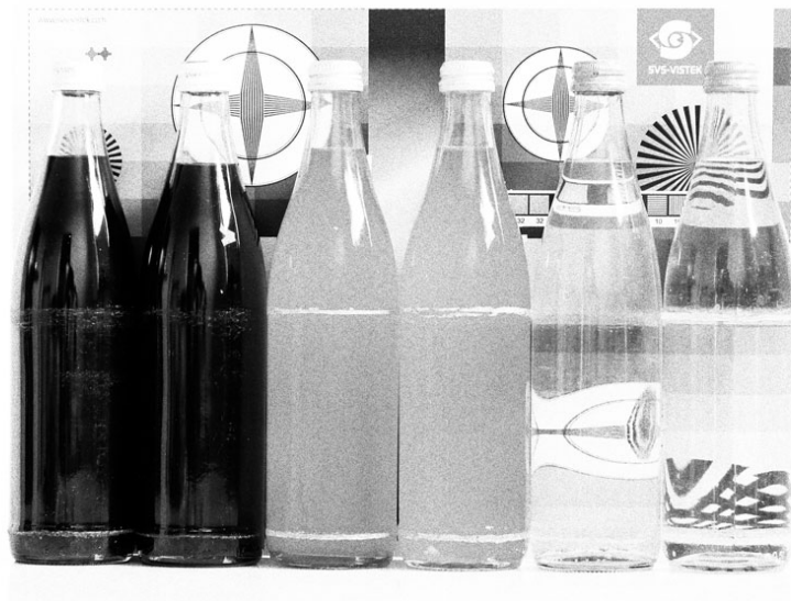
Figure 31: noise caused by increasing gain excessively
