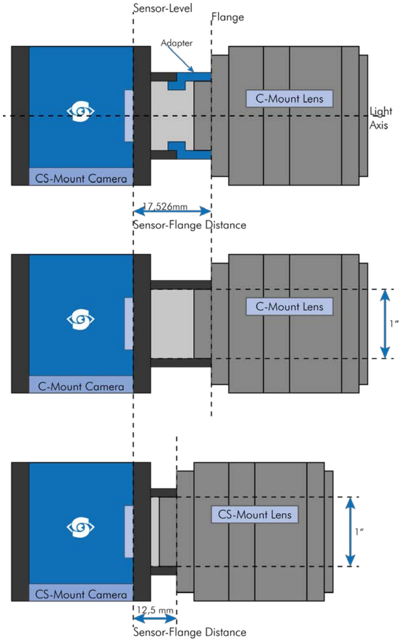
Figure 13: Illustration of C- & CS-Mount differences
