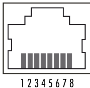
Figure 7: Illustration of RJ45 female connector
