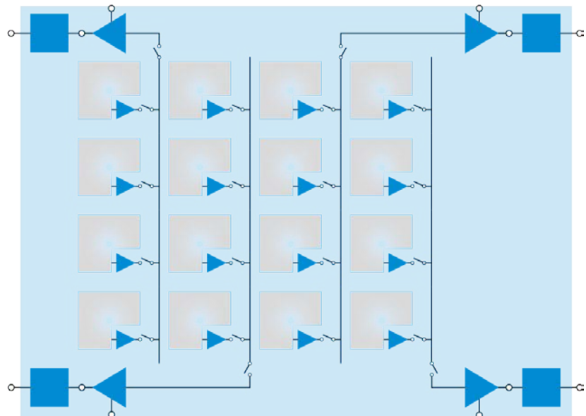
Figure 16: Illustration of CMOS four channel output Actual readout order differs from sensor to sensor.
