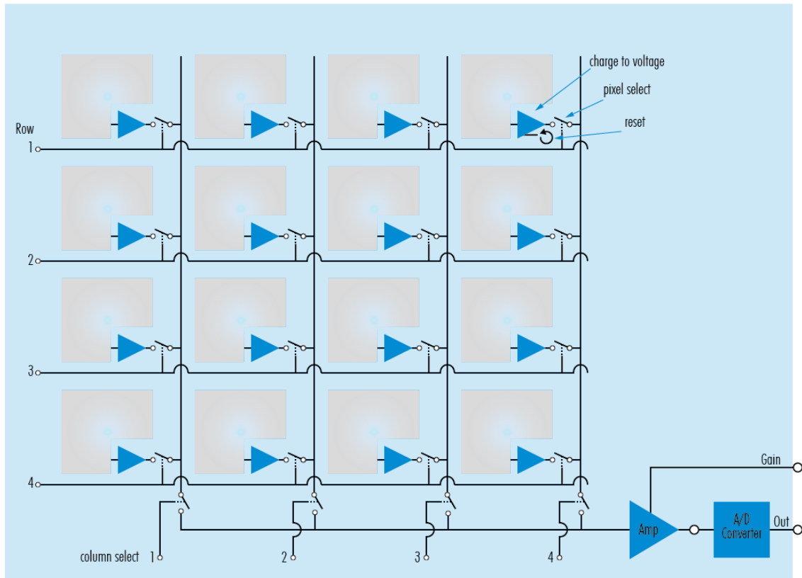
Figure 15: Illustration of CMOS on chip processing
