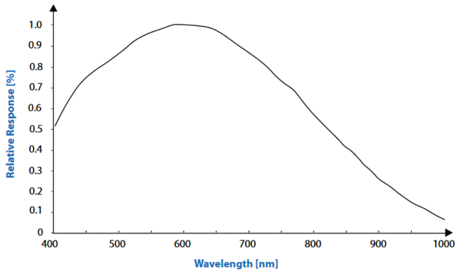
Figure 74: IMX264LLR spectral response
