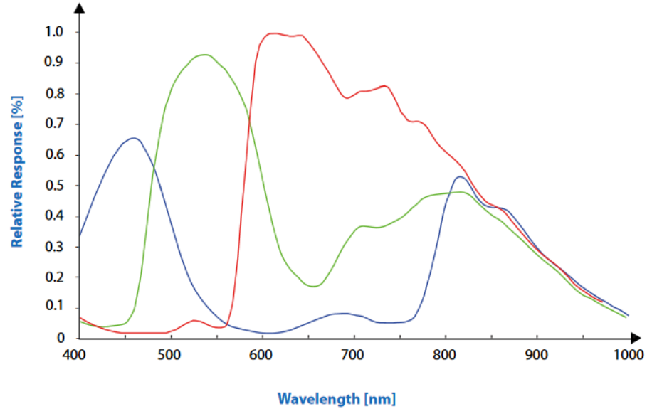
Figure 73: IMX264LQR spectral response
