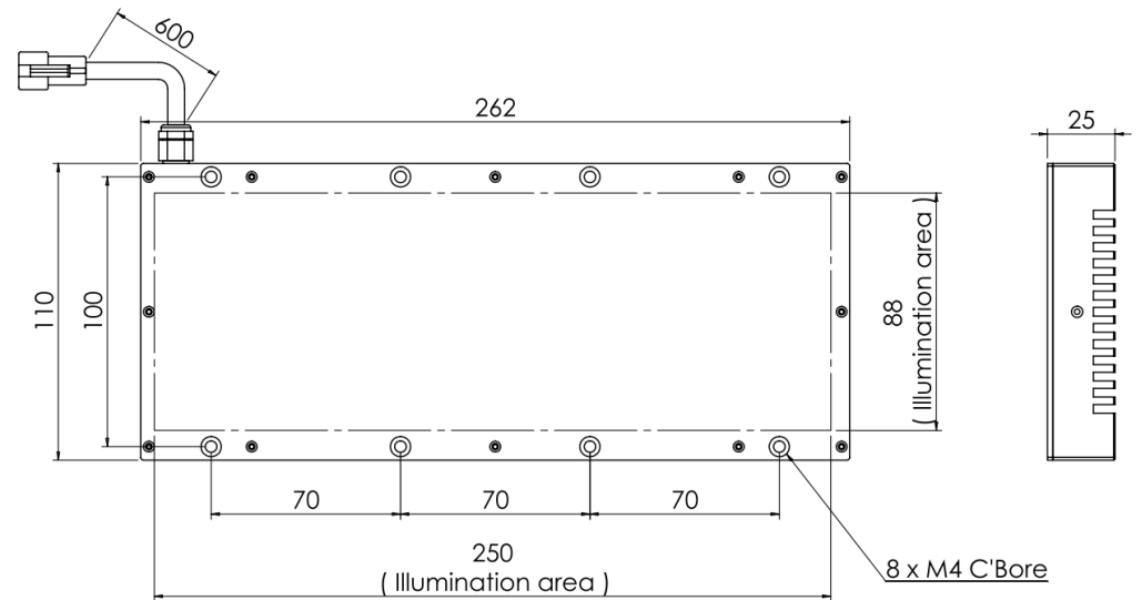
Lighting Dimension
