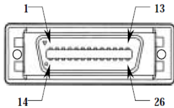
Pin Assignment
