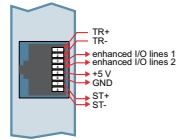
System connector RJ45
