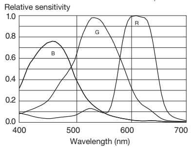
• XCL-C280C (Lens characteristics and light source characteristics excluded.)
