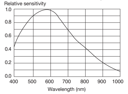
• XCL-C130 (Lens characteristics and light source characteristics excluded.)
