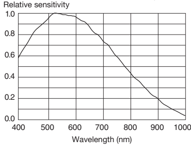
• XCL-C280 (Lens characteristics and light source characteristics excluded.)
