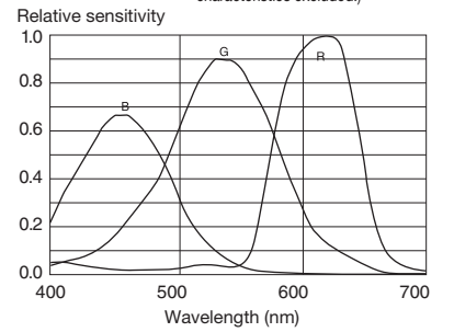
• XCL-C130C (Lens characteristics and light source characteristics excluded.)
