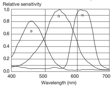
• XCL-C500C (Lens characteristics and light source characteristics excluded.)
