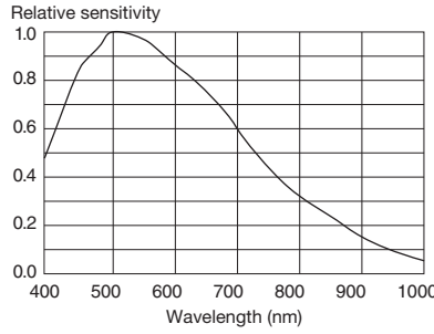
• XCL-C500 (Lens characteristics and light source characteristics excluded.)
