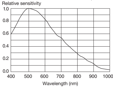
• XCL-C30 (Lens characteristics and light source characteristics excluded.)
