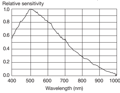
• XCL-C32 (Lens characteristics and light source characteristics excluded.)
