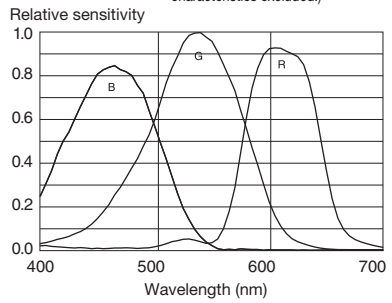
• XCL-C32C (Lens characteristics and light source characteristics excluded.)
